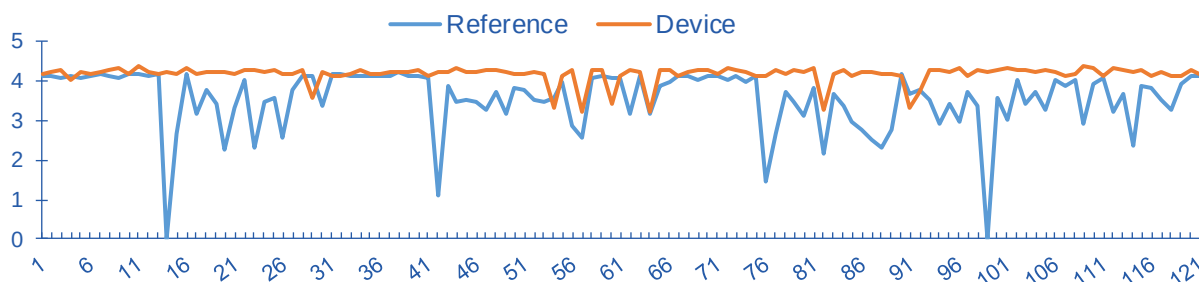
Multi Handover Linksys Hydra Pro 6E - Profile 2 MOS Scores
