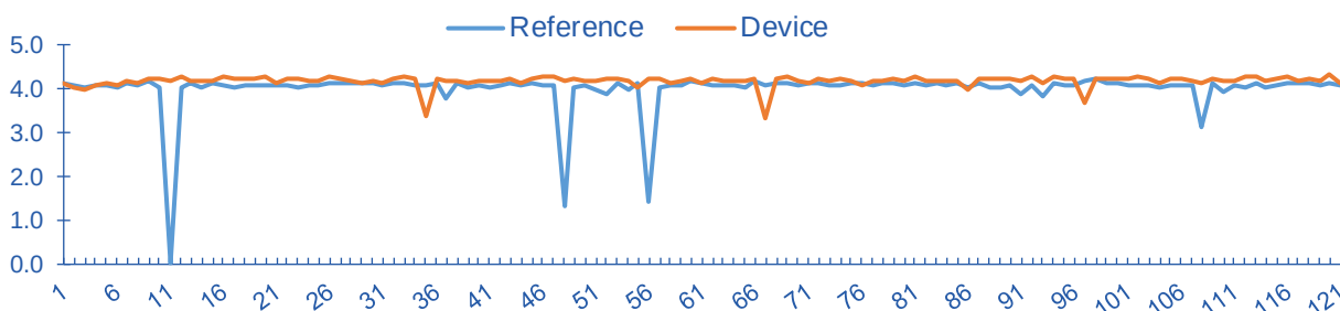
Multi Handover 5G21-12W-A (Nokia) - Profile 2 MOS Scores
