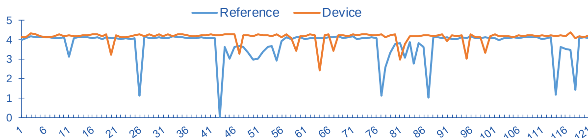
Multi Handover Linksys Hydra Pro 6E - Profile 1 MOS Scores
