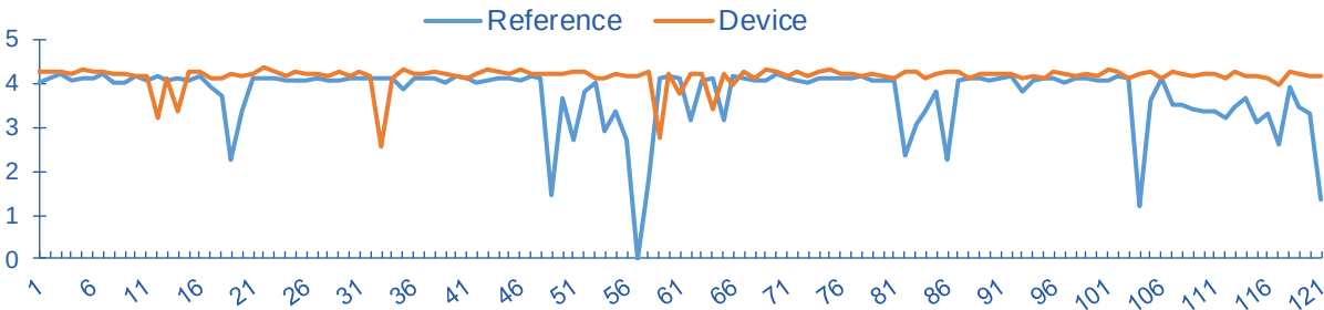
Multi Handover ASUS RT-AC68U - Profile 2 MOS Scores
