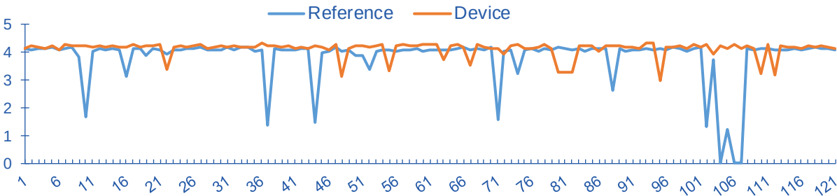
Multi Handover ASUS RT-AC68U - Profile 3 MOS Scores
