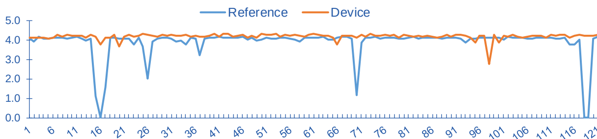
Multi Handover 5G21-12W-A (Nokia) - Profile 1 MOS Scores
