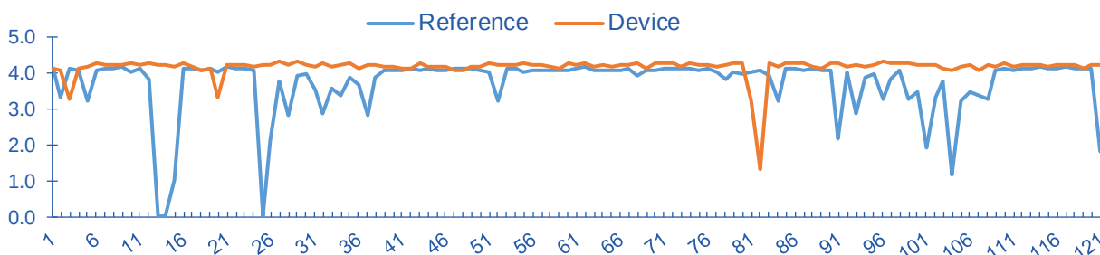
Multi Handover 5G21-12W-A (Nokia) - Profile 3 MOS Scores
